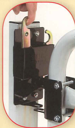
Lockable Two-Way Livestock Gate Latch
